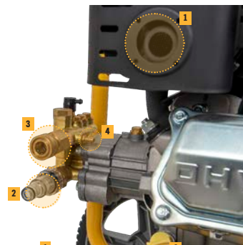
Exhaust and water inlet filter, High pressure coupling and detergent hose connector.
